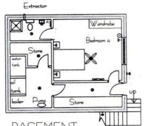
BASEMENT
