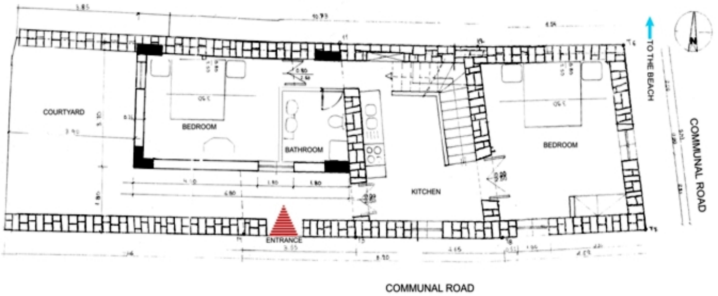
GROUND FLOOR: 79m 2
